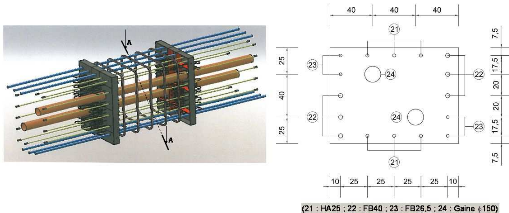
Figure 2 - Reinforcement of the "zone of interest"
