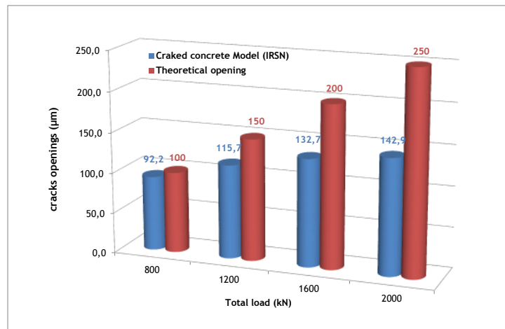
Figure 12 - Cracks openings as a function of the total load applied by the jacks
