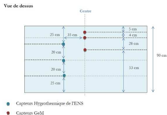
Location of the hygrothermal sensors
