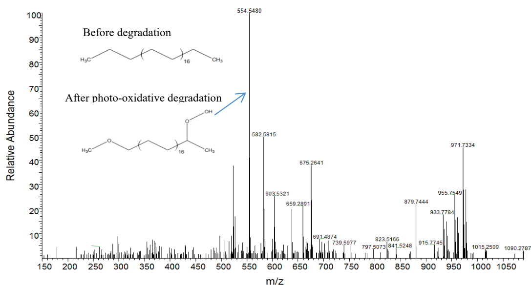
Figure 3. LESA-MS spectrum of an oxidized low-quality low-density polyethylene (LDPE). (Reprinted from [36] with permission of Elsevier).
