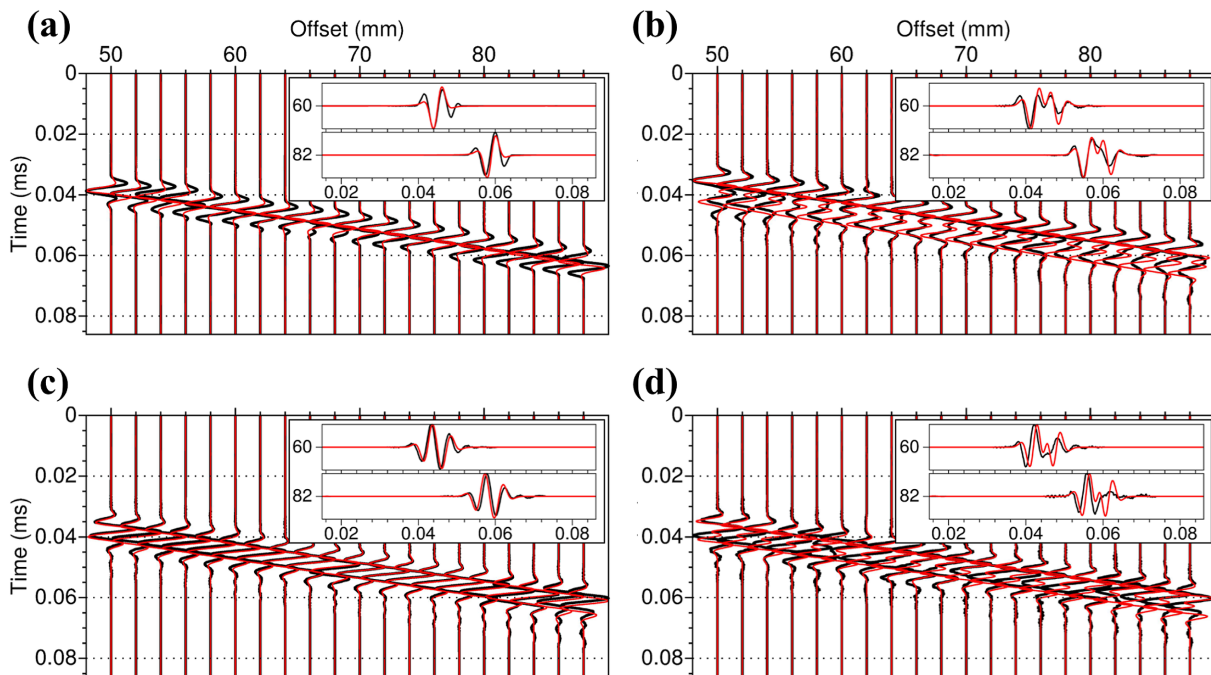
Figure 11. Comparisons between laboratory data (black) and numerical simulations (red) for the P -direct waves arriving propagating in material 1 with an angle \alpha \simeq 40^\circ . (a) Vertical seismic acceleration. Seismoelectric data are displayed for two-electrode (b), three-electrode (c) and five-electrode (d) arrangements. The insets zoom in at two acquisition offsets: 60 and 82 mm.
