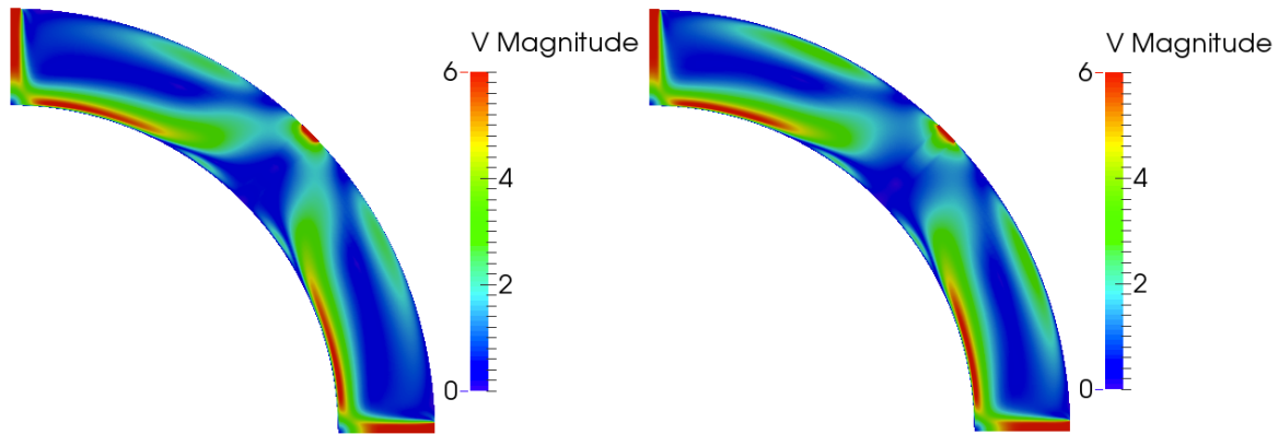
Fig. 13a. Left: Velocity inside the cavity by elsA +Jameson.
