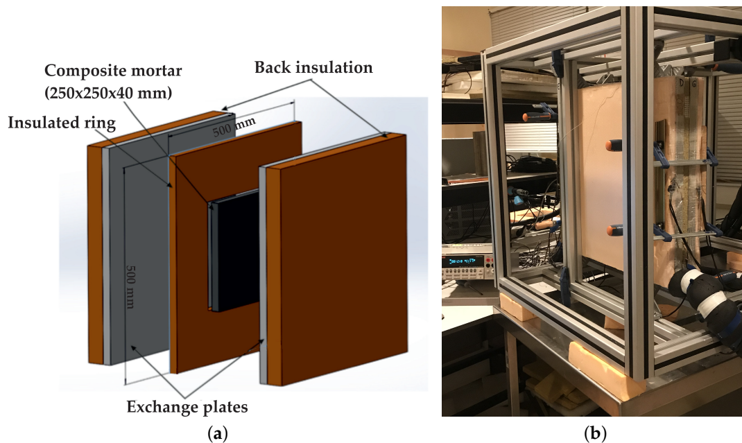
Figure 2. Schematic view of the experimental set-up. (a) Exploded view; (b) Real picture.
