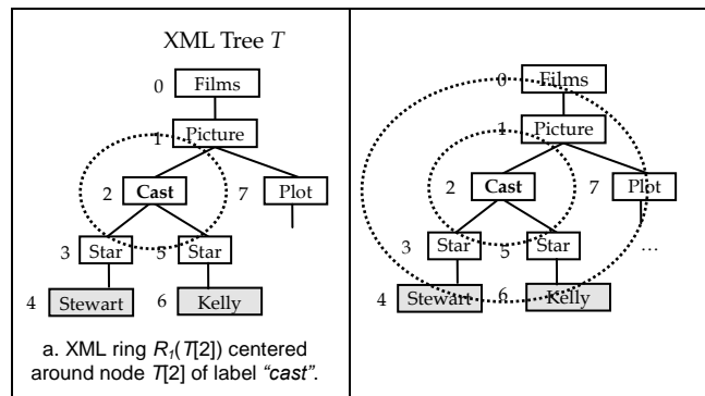
Fig. 6. Sample XML context (ring and) sphere neighborhoods.
