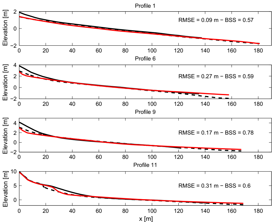
Fig. 5 Beach profiles measured before ( black solid line ) and after ( black dashed line ) a series of storms (Table 1) and the profiles computed with XBeach ( red solid line ) at four locations along the beach
