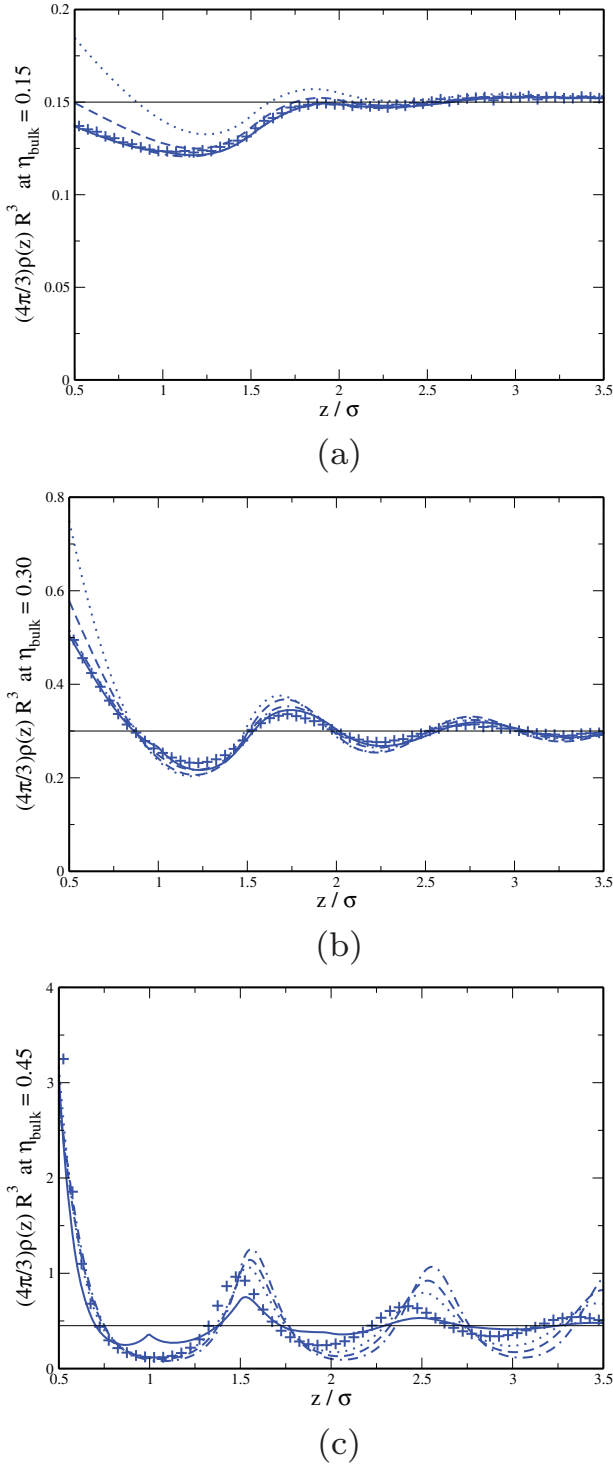
Figure 4. Density profiles of the pure square-well fluid studied. The variable z represents the normal distance to the left hard planar wall placed at z = 0 . (a) \eta_{\text{bulk}} = 0.15 ; (b) \eta_{\text{bulk}} = 0.30 ; (c) \eta_{\text{bulk}} = 0.45 .
