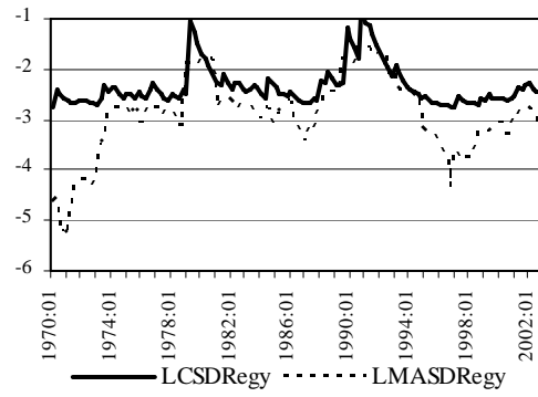
Figure 2. Log of volatility - REER Egypt -
