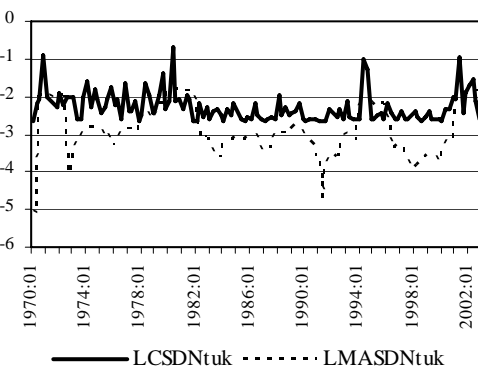
Figure 12. Log of volatility -NEER Turkey-
