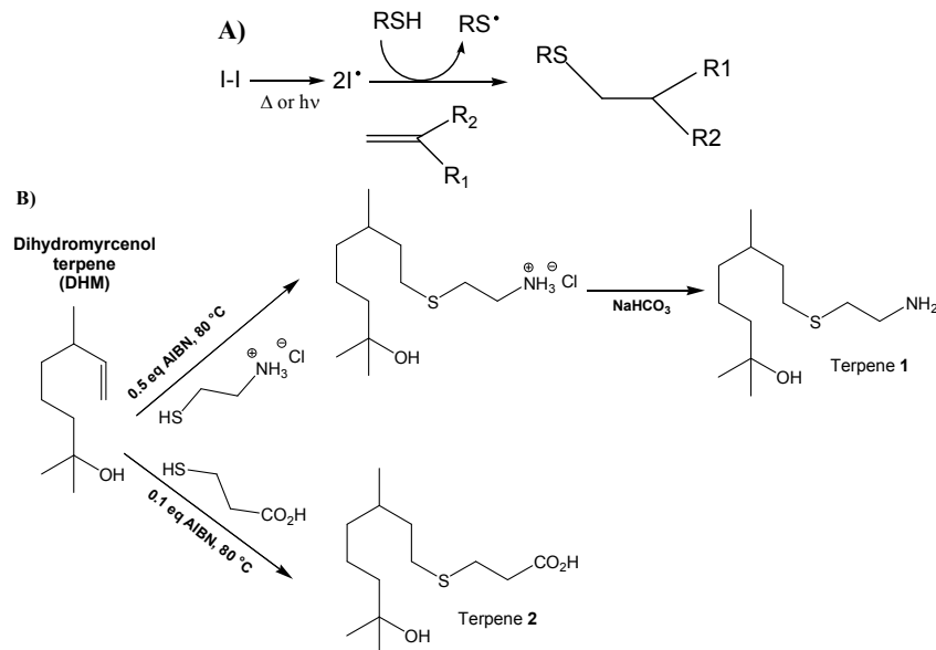
43 44 45 46 47 48 49 50 51 Scheme 2. (A) General principle of radical thiol-ene chemistry using an initiator (I-I) and a thiol transfer agent (RSH); (B) Derivatization of dihydromyrcenol (DHM) terpene by thiol-ene chemistry to produce functional Terpene 1 and Terpene 2.
