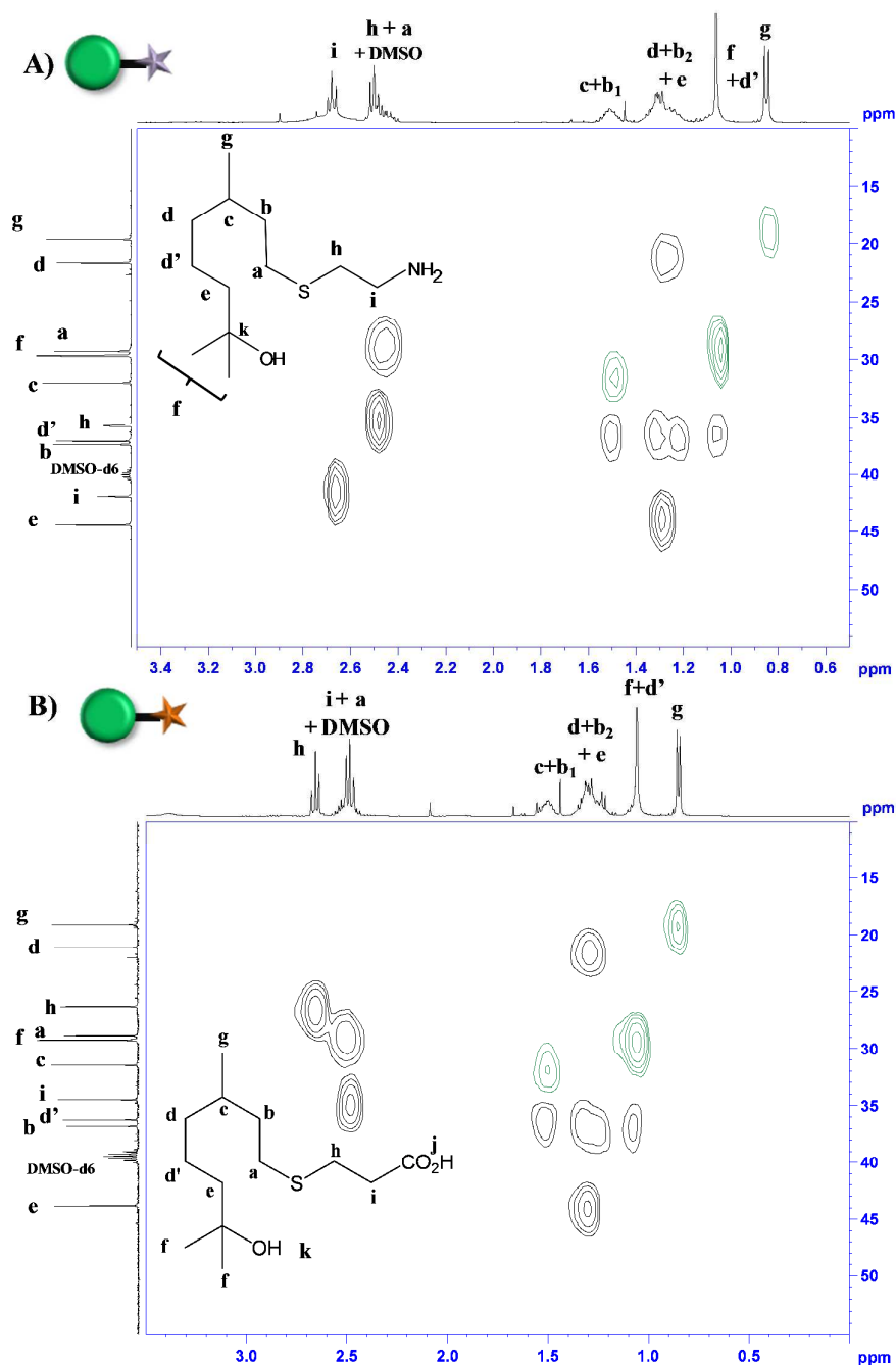
Figure 3. HSQC spectra of Terpene 1 (A) and Terpene 2 (B) in DMSO- d 6 .
